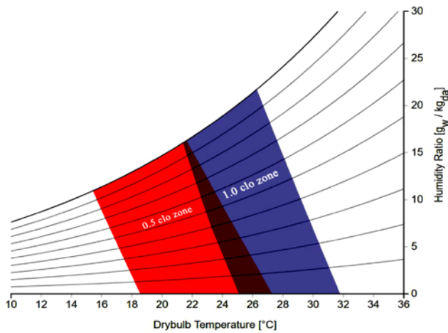
Figure 6. ASHRAE comfort condition range.
