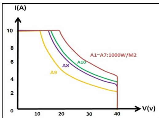
Figure 9. Panels I-V Characteristics of string A
