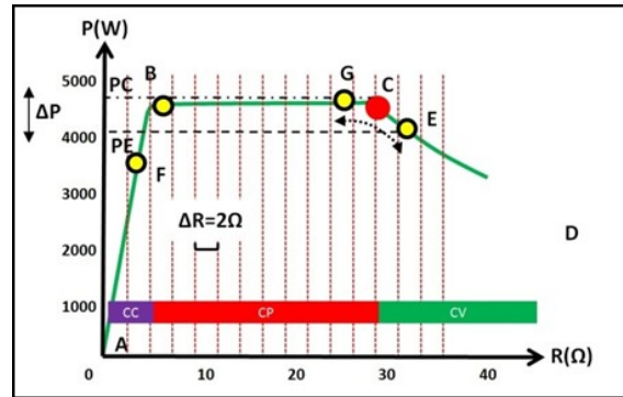
Figure 16. Steady state operation of conductance control MPPT
