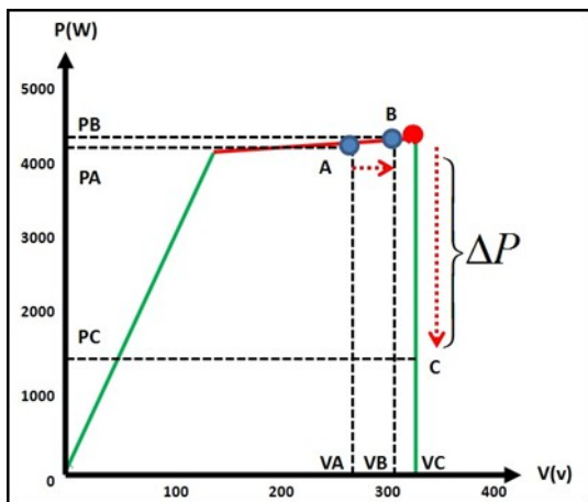
Figure 12. Voltage control instability
