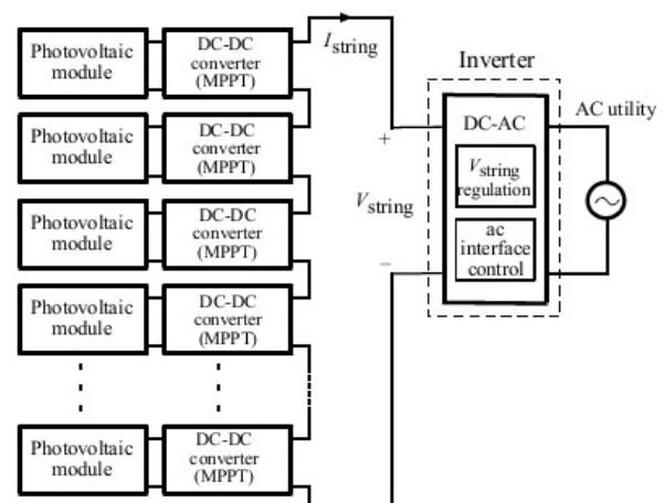
Figure 1. Block diagram of intelligent
