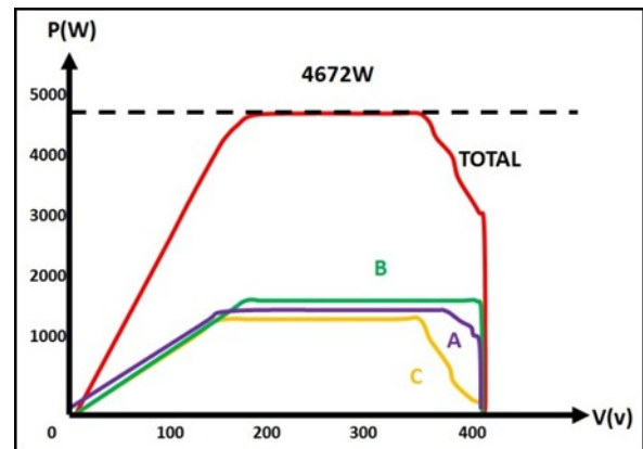
Figure 11. Output P-V of A, B, C and array output P-V
