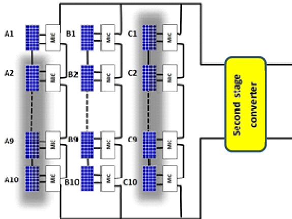
Figure 7. Case study arranged with intelligent structure
