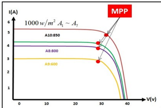
Figure 4. Current versus voltage in string A panels
