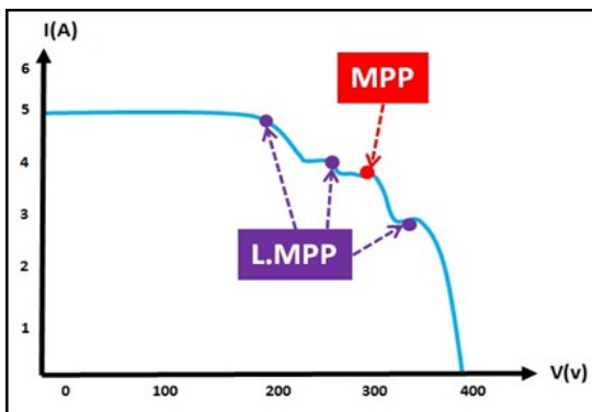
Figure 5. Output current versus voltage string A
