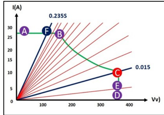
Figure 13. Representation of conductance control MPPT with constant step size
