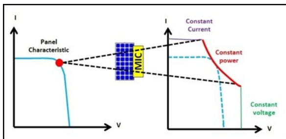
Figure 8. Input & output characteristics of single intelligent converter
