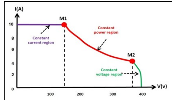
Figure 10. Composite output of string A
