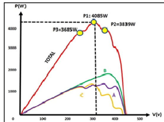
Figure 6. P-V characteristics curve of string A, B, C and total arrays
