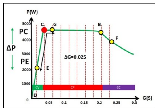
Figure 14. Steady state operation of conductance control MPPT
