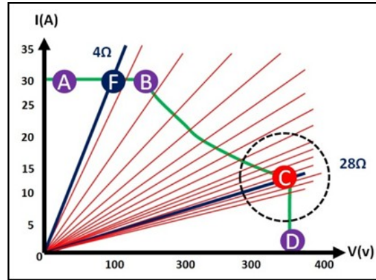
Figure 15. Representation of resistance control MPPT with constant step size
