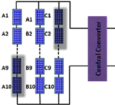
Figure 3. case study arranged with central structure (Shaded A8 and C5 missing – use of foreign language!)
