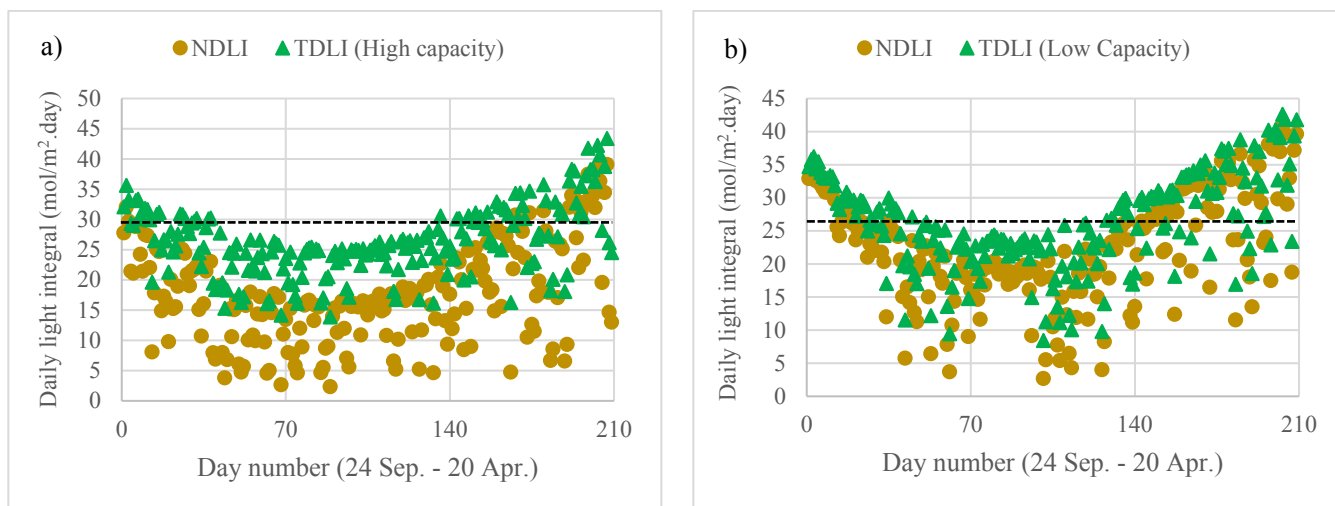
Figure 15. Natural daily light integral and Total Daily Light Integral (TDLI) for Venlo structure in two different artificial light capacities of a) 200 \mu\text{mol m}^{-2} \text{s}^{-1} and b) 100 \mu\text{mol m}^{-2} \text{s}^{-1} in Rasht
