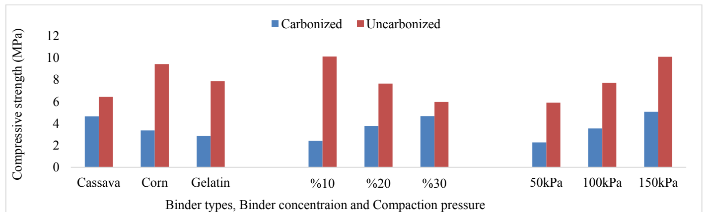
Figure 6. Compressive strength of the briquettes as affected by processing parameters
