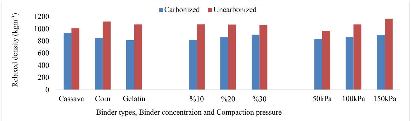
Figure 5. Relaxed density of the briquettes as affected by processing parameters
