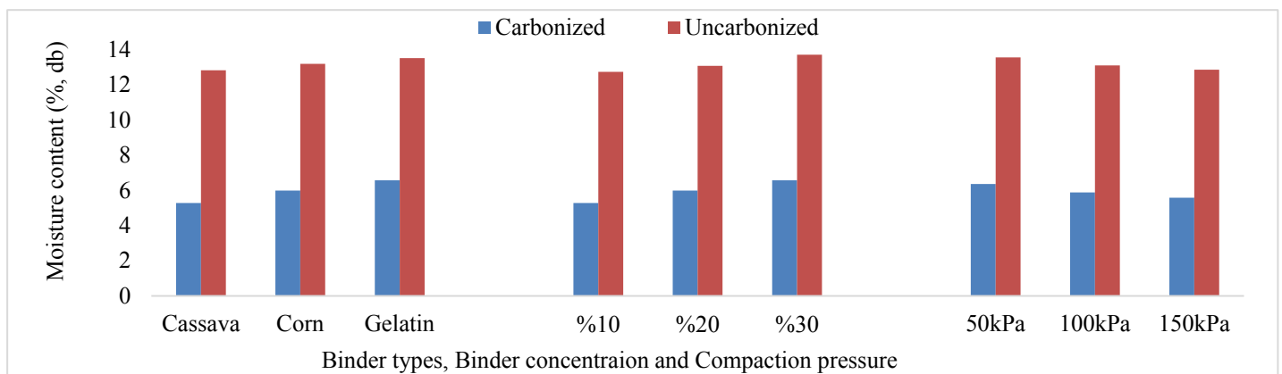
Figure 3. Moisture content of the briquettes as affected by processing parameters
