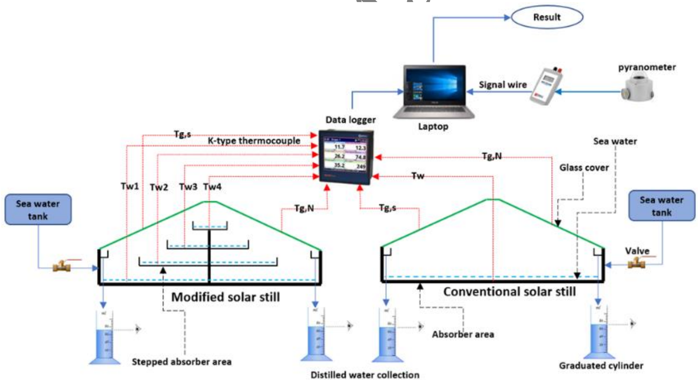
Figure 1 Schematic diagram of the proposed system.
