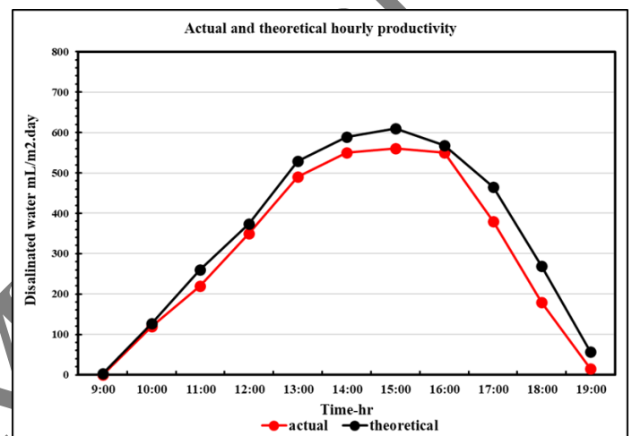
Figure 9. Theoretical/experimental results of distillate output.
