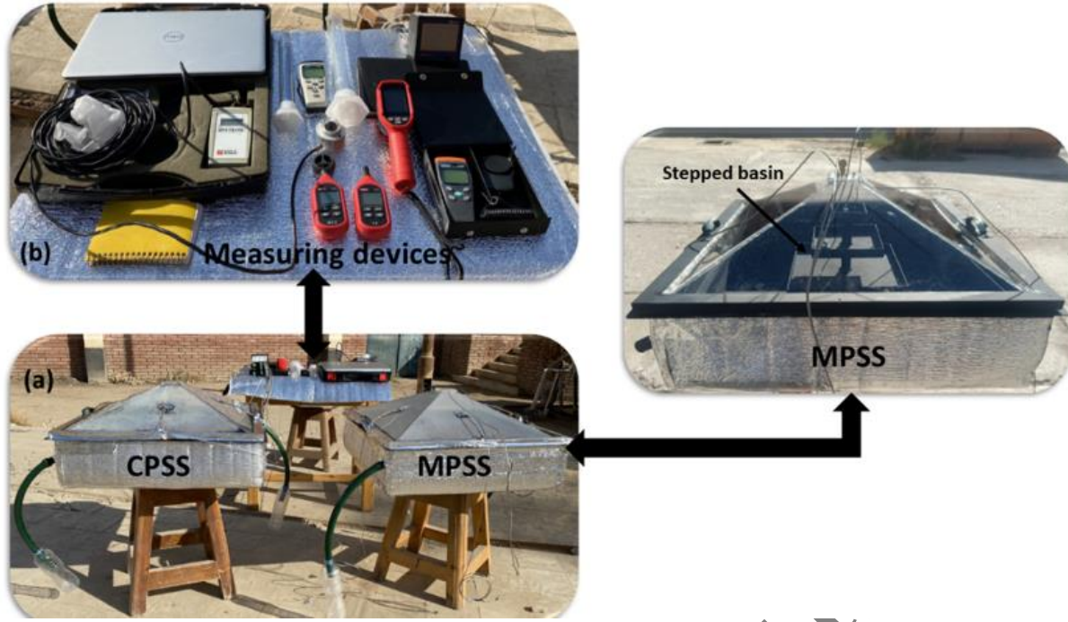
Figure 2 (a) Experimental test rig, (b) measuring devices.
