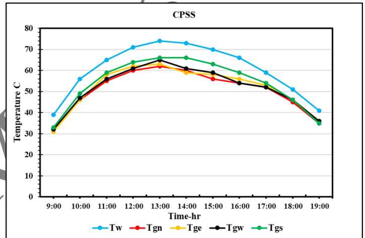
Figure 5. Variation between water and condensing cover temperatures in CPSS.
