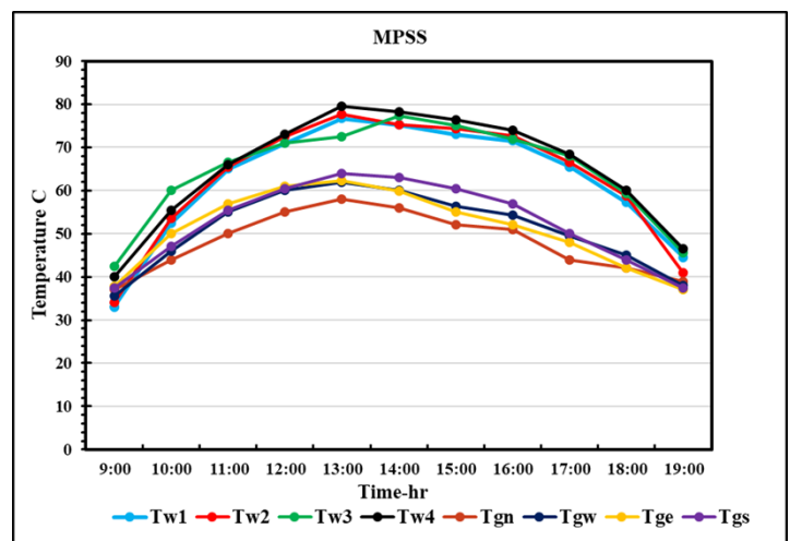
Figure 6. Variation between water and condensing cover temperatures in MPSS.
