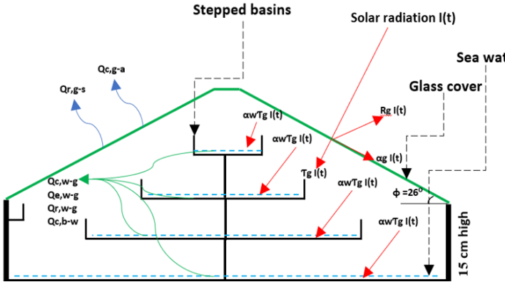
Figure 3 Schematic of the heat flow through the parts of MPSS.
