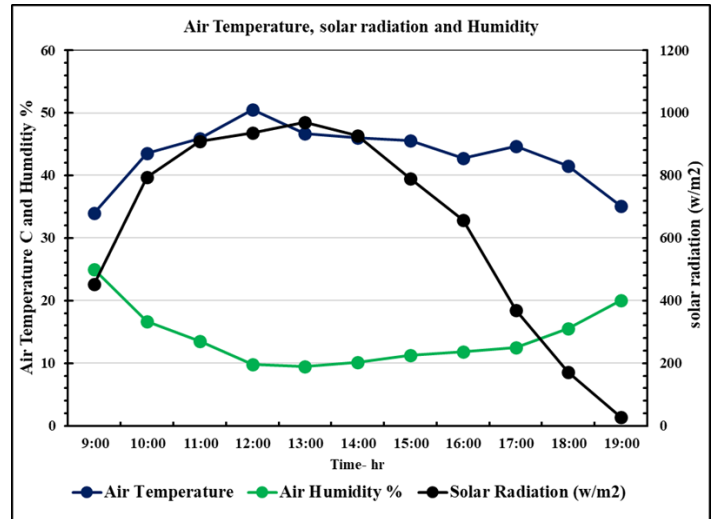
Figure 4. Variation between outside condition with time.
