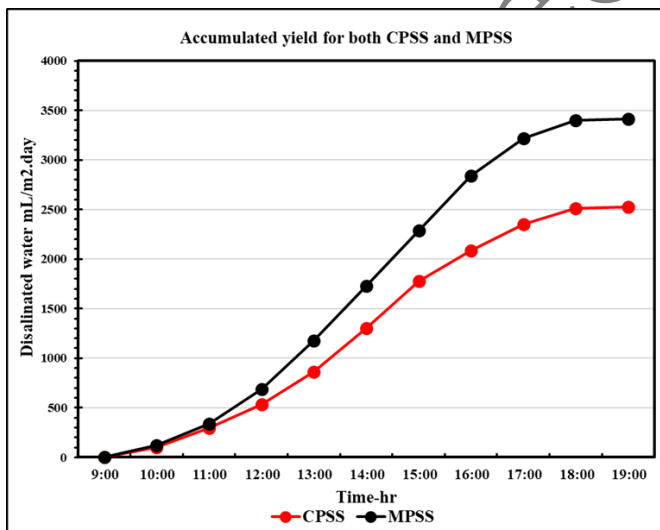
Figure 8. Variation between accumulated yield in CPSS and MPSS with time.
