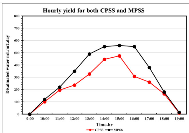
Figure 7. Variation between hourly yield in CPSS and MPSS with time.
