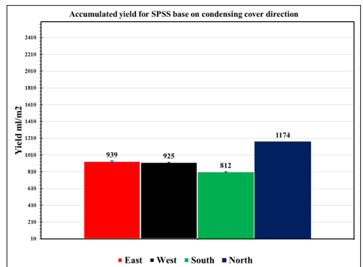
Figure 10. Maximum yield of freshwater based on condensing cover direction.
