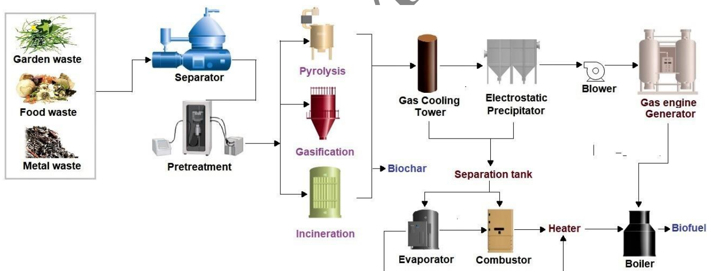
Figure 6. Thermal conversion of organic fraction of municipal solid waste
