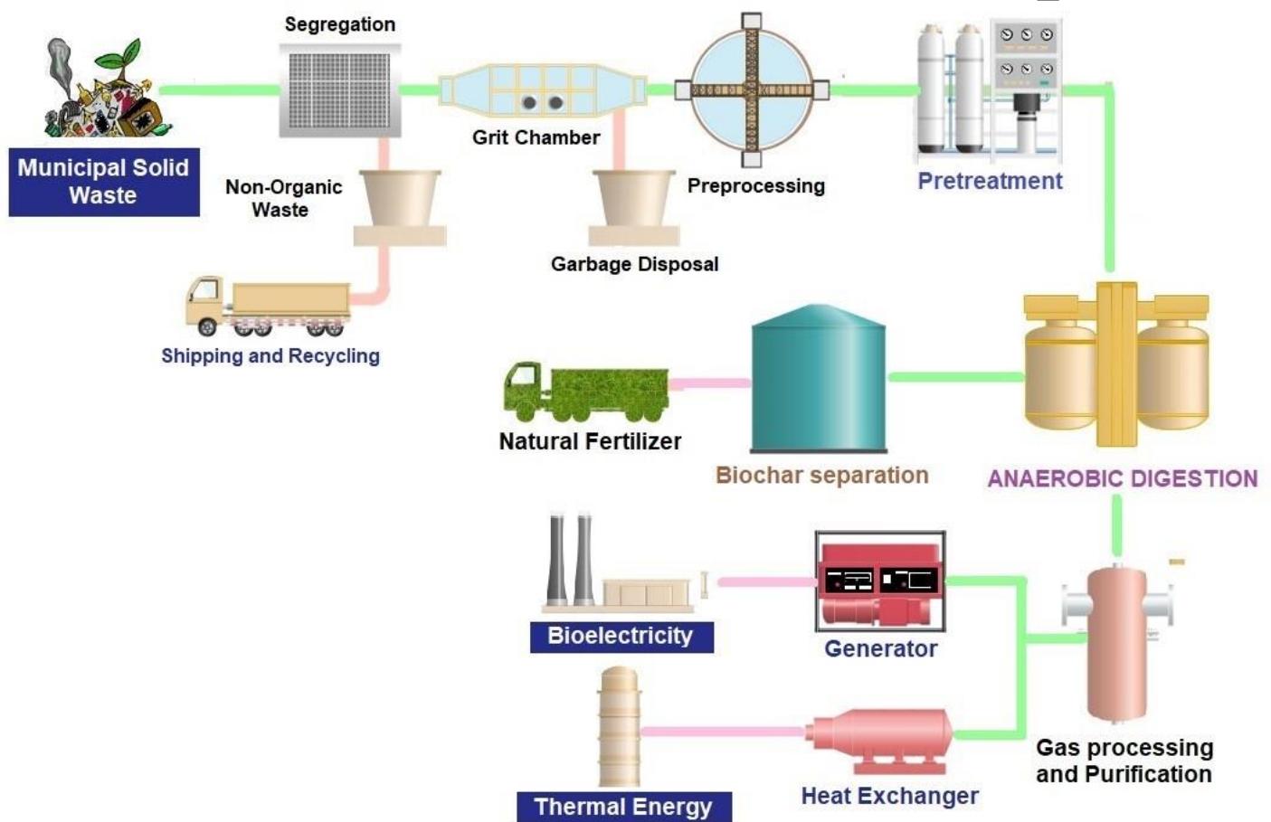
Figure 7. Steps involved in anaerobic digestion based treatment of municipal solid waste
